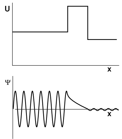
n / Tunneling through a barrier. (As discussed on p. 864, it is actually not quite correct to graph the wavefunction of an electron as a real number unless it is a standing wave, which isn't the case here.)
